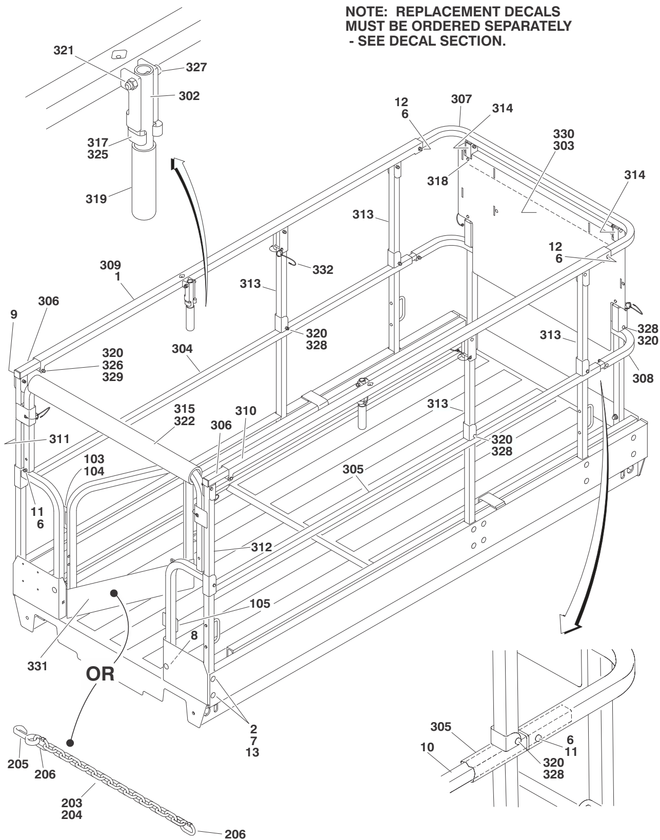
FIGURE 4-5.RAIL INSTALLATION - 2646ES/3246ES
