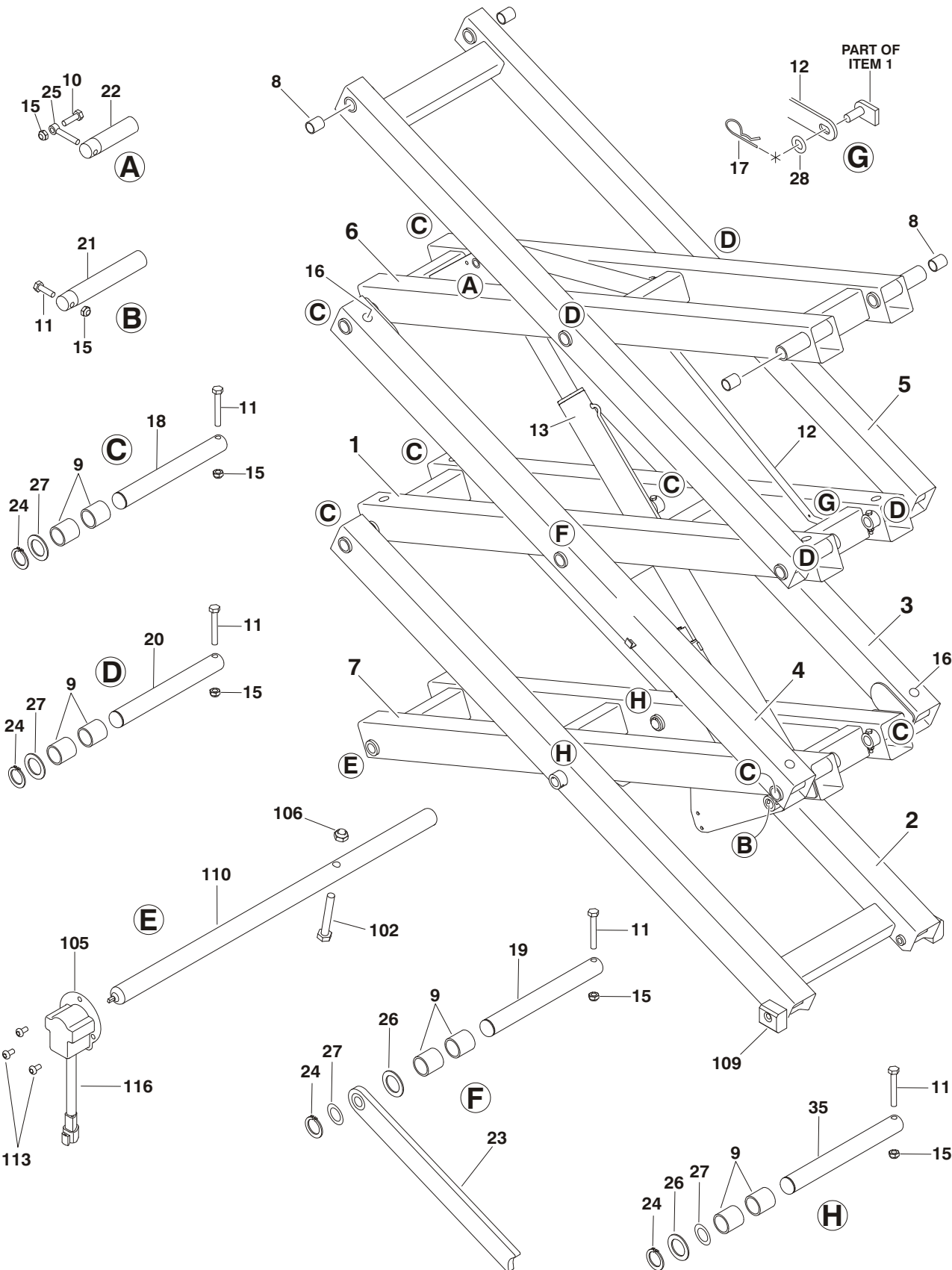
FIGURE 3-2.SCISSOR ARMS INSTALLATION - 2030ES
