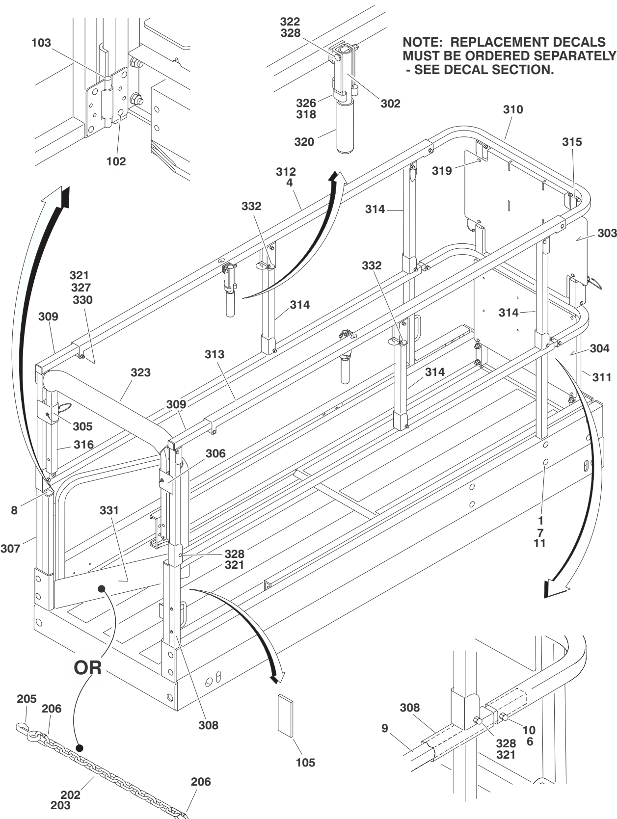
FIGURE 4-4.RAIL INSTALLATION - 2030ES/2630ES
